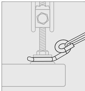
Loop wire through the hook
